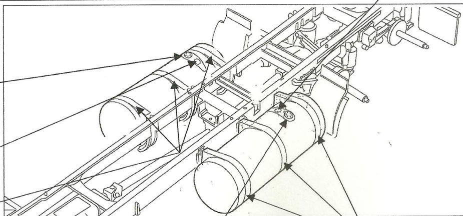
10/Fuel tank cap
