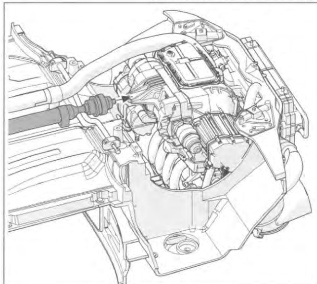
DRIVE SHAFT - ENGINE ASSEMBLY
